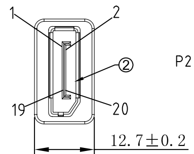
DISPLAYPORT FEMALE
